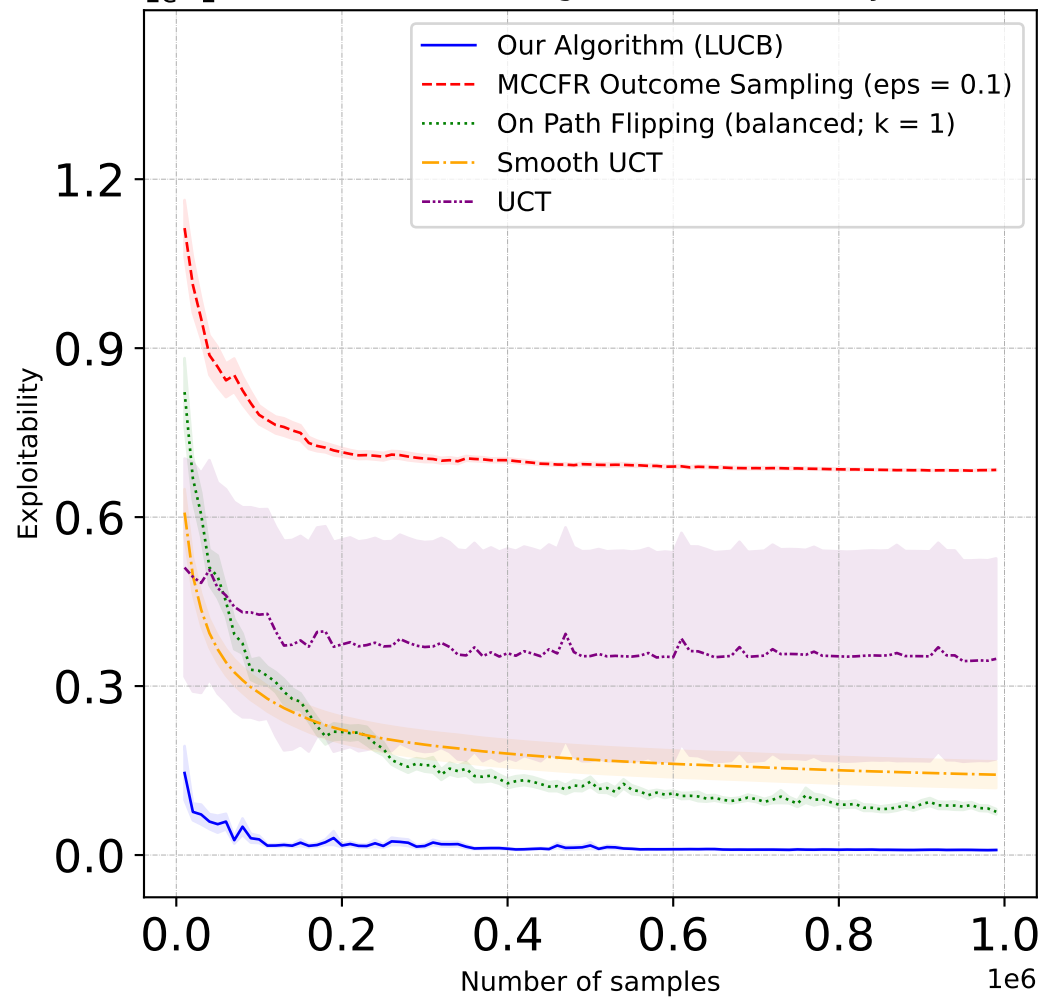
1e-1 Leduc Poker, Best Algorithms (new), Player o
